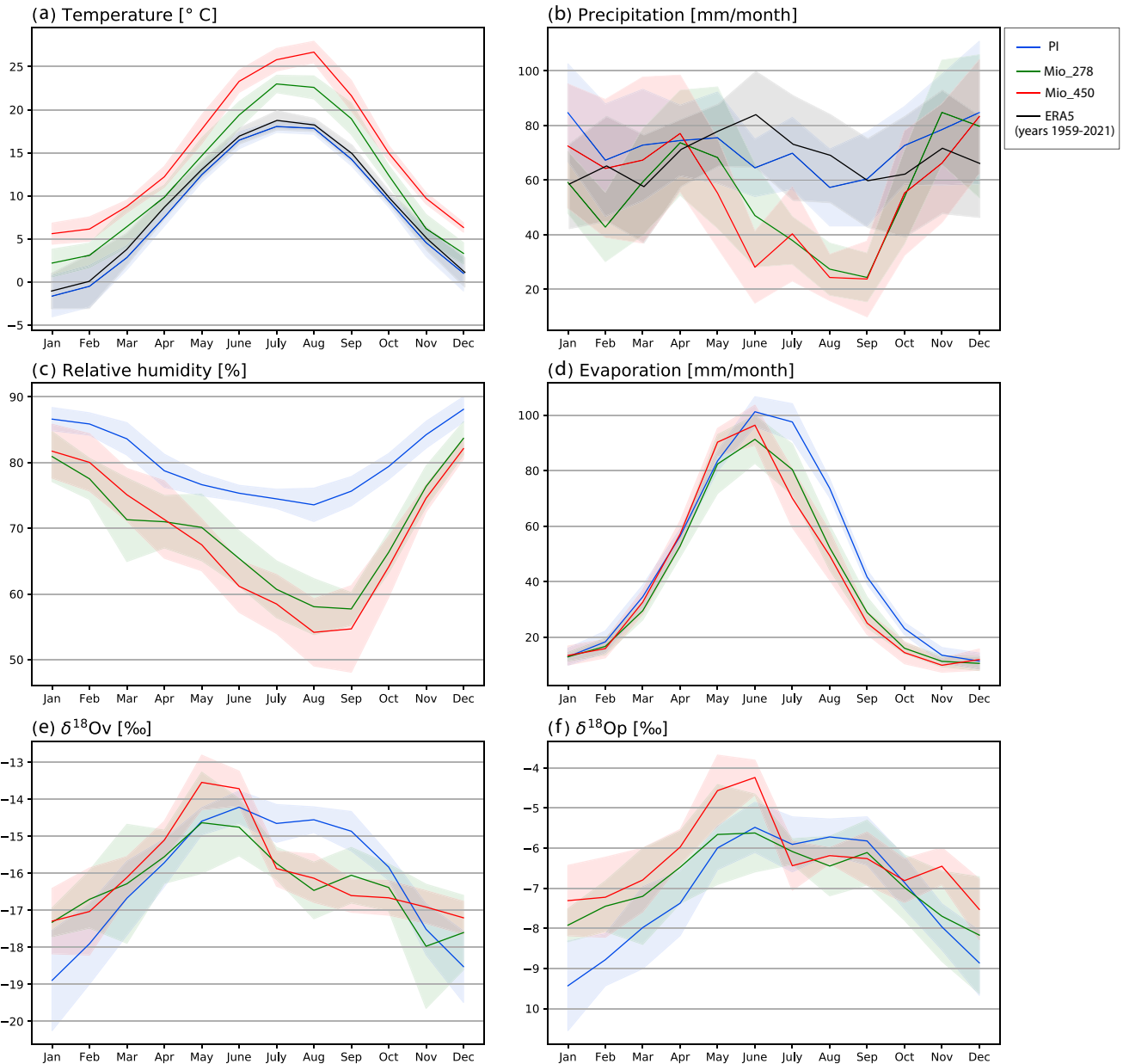
Figure 9. Intra-annual variations of (a) near-surface temperature, (b) total precipitation, (c) low-level relative humidity, (d) surface evaporation, (e) \delta^{18}O_v values, and (f) \delta^{18}O_p values. All variables are averaged for continental central Europe. Blue color corresponds to the PI experiment, green—Mio_278 experiment, red—Mio_450 experiment, black—ERA5 reanalysis from 1959 to 2021. Solid lines show multi-annual mean, shade shows interannual variability within one standard deviation for the corresponding variable.
